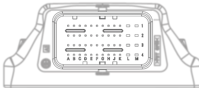
48 PINS CONNECTOR PINOUT TABLE
